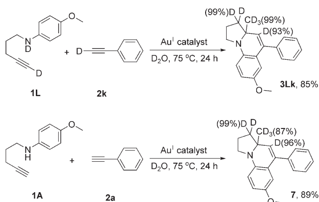
Scheme 5. Labeling studies with deuterated starting materials or D_2O . Au I catalyst = [Au\{P(tBu)_2(o\text{-biphenyl})\}]Cl/AgSbF_6 .
